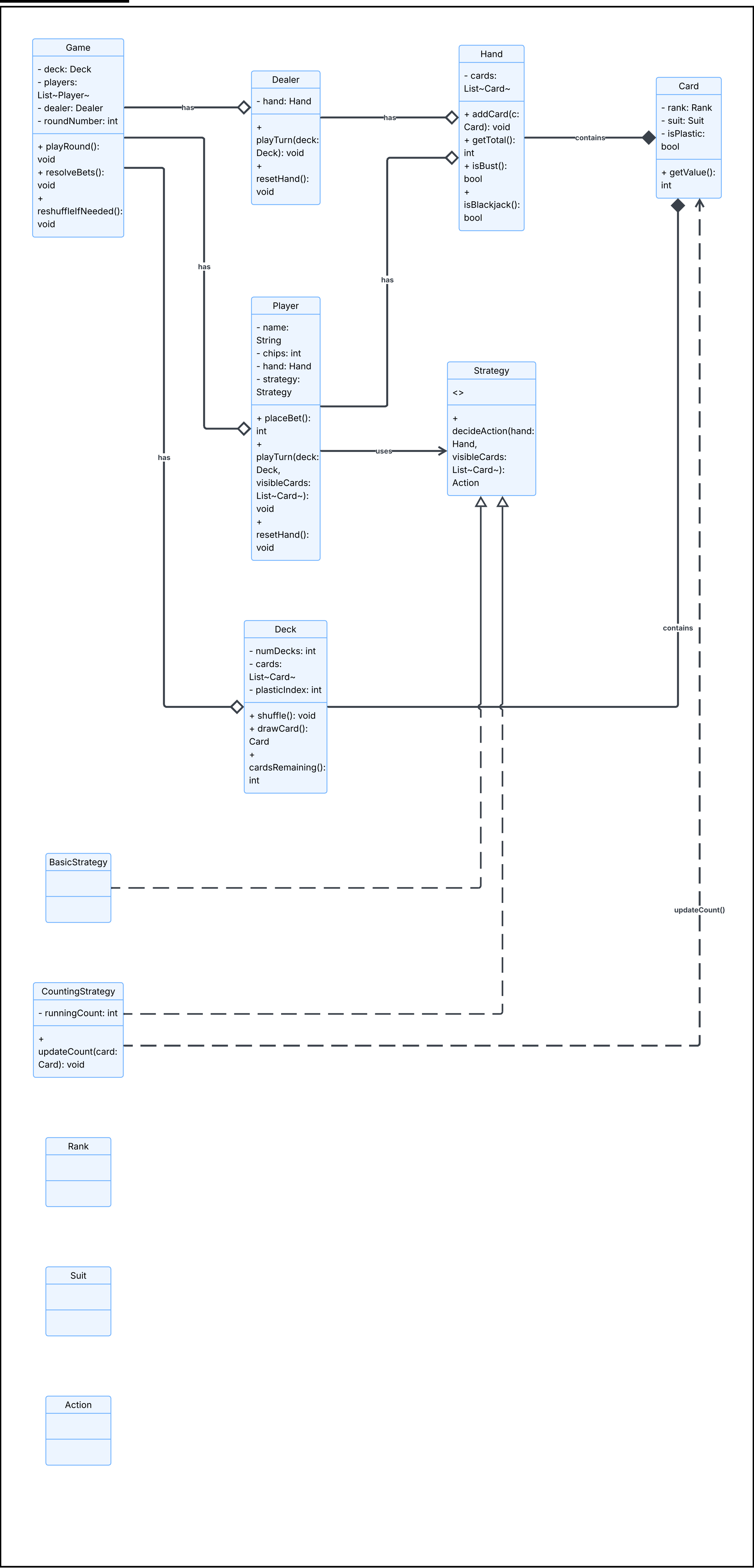
Blackjack Game System UML Diagram
